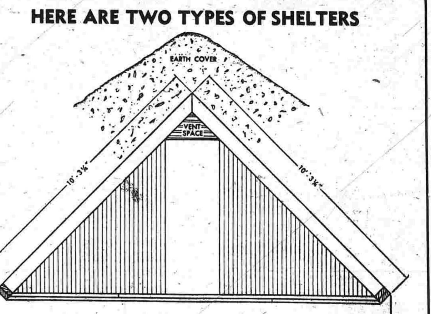
Above ground shelter built of 2"x8" wood joist, waterproofed and covered with earth. This is the front elevation.
