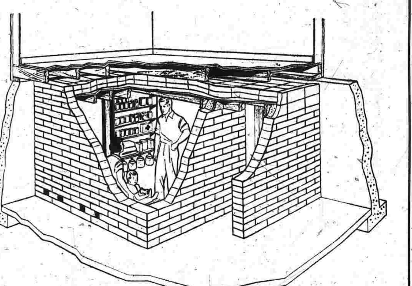
The Basement Shelter Which Can Be Cement Block, Brick or Concrete
